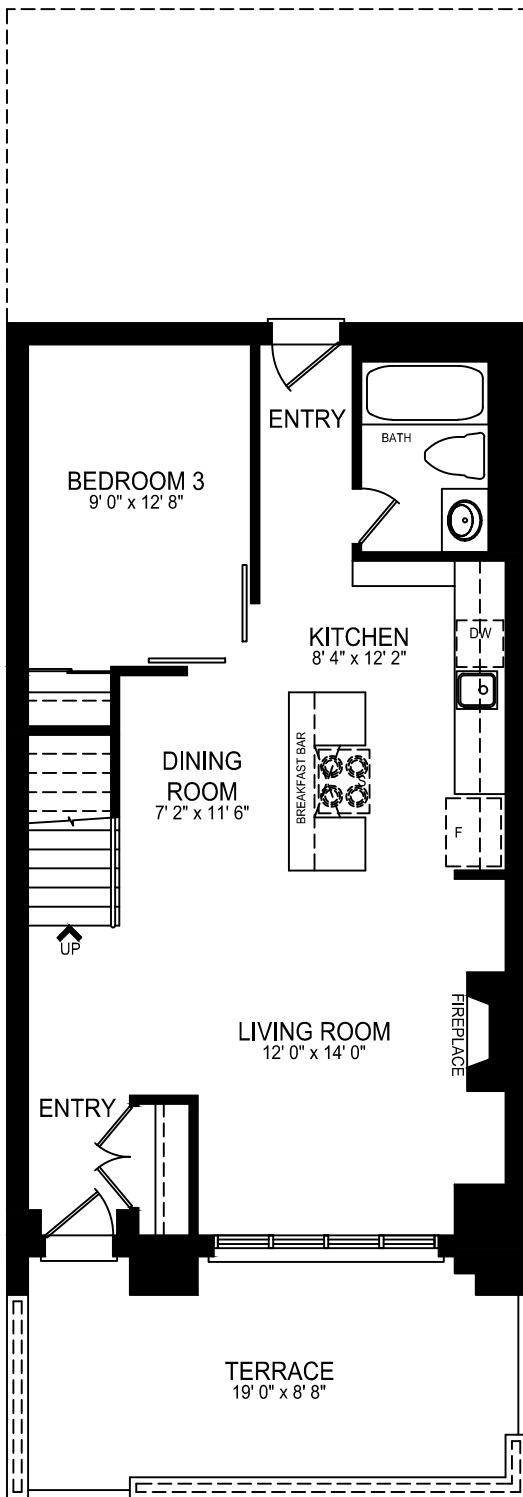
GROUND FLOOR PLAN APPROX. 764 SQ.FT.
