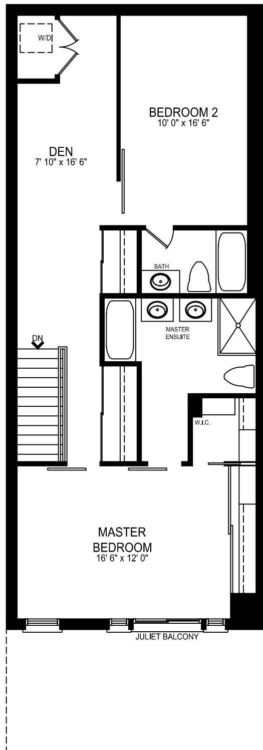
SECOND FLOOR PLAN APPROX. 1,003 SQ.FT.
