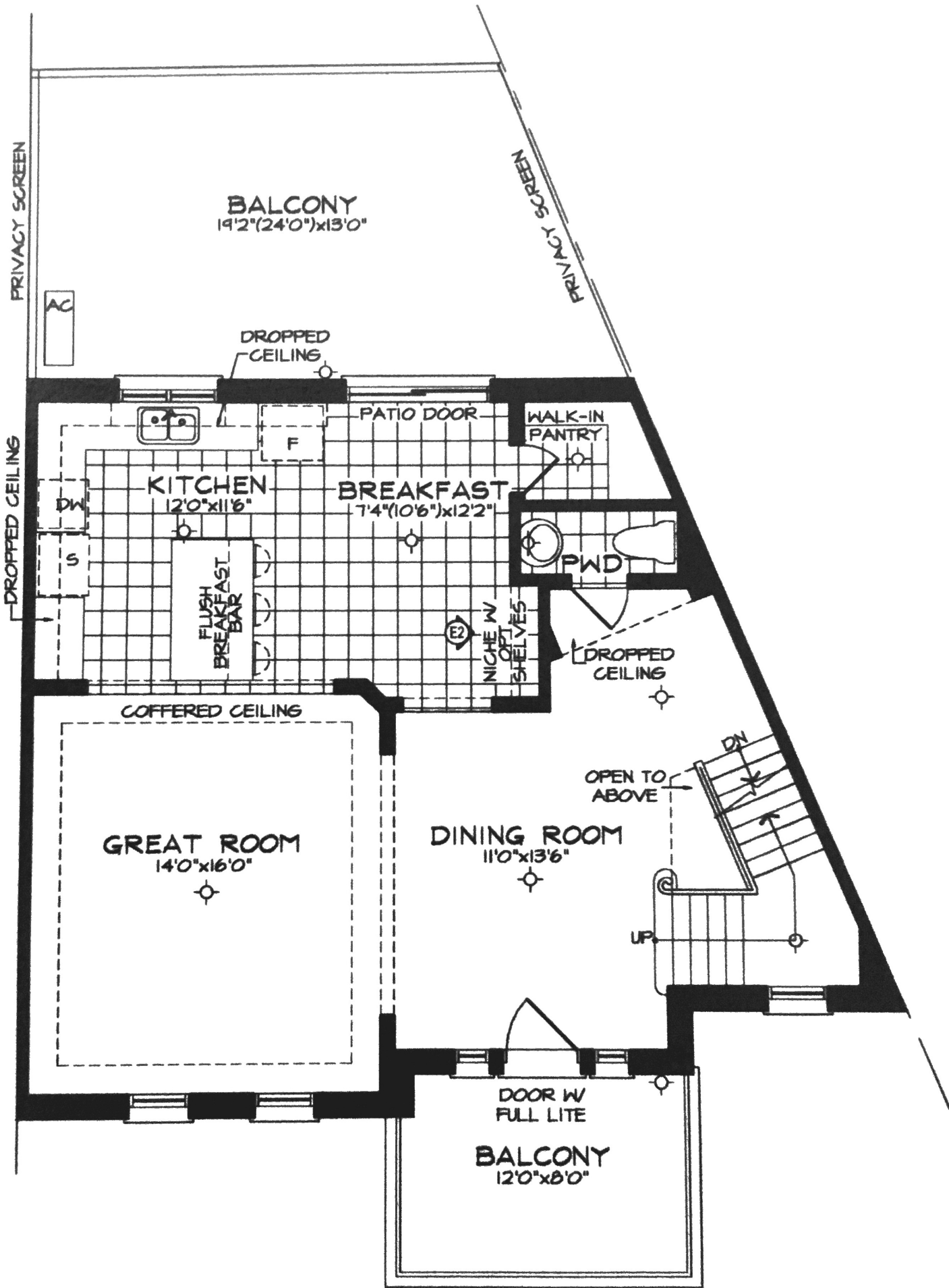
SECOND FLOOR PLAN 'D2'
