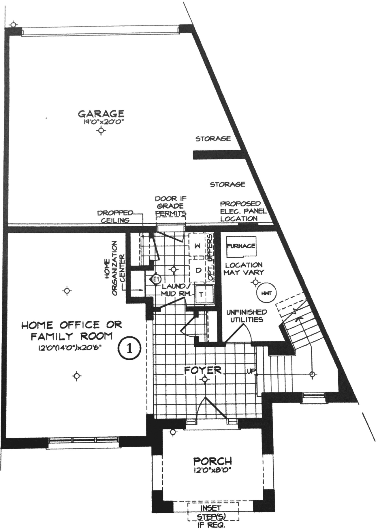
GROUND FLOOR PLAN 'D2'
