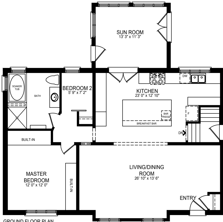
GROUND FLOOR PLAN APPROX. 1,295 SQ.FT.
