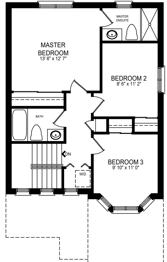
SECOND FLOOR PLAN APPROX. 720 SQ.FT.
