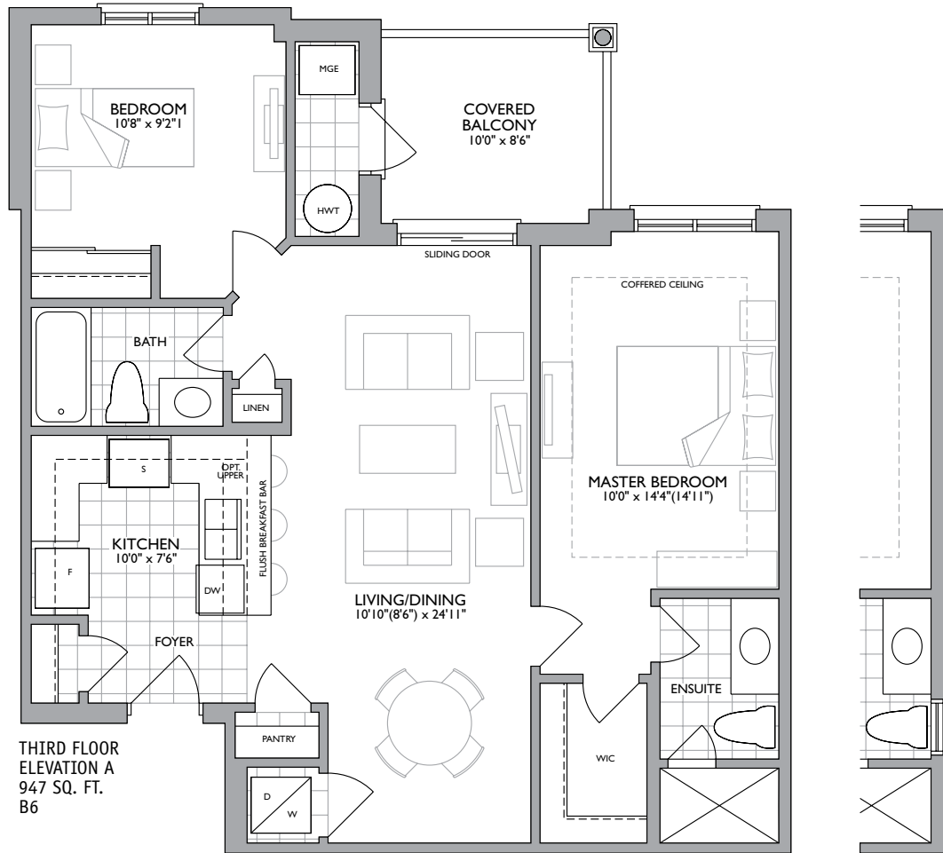
THIRD FLOOR ELEVATION A END 958 SQ. FT. B2, B3, B5
